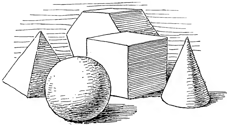
ELEMENTARY FORMS: PYRAMID, SPHERE, CUBE, HEXAGON, CONE.
